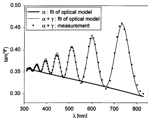
Figure 3. Wavelength dependence of \tan(\Psi) for the \gamma -alumina layer on top of the \alpha -alumina layer.
